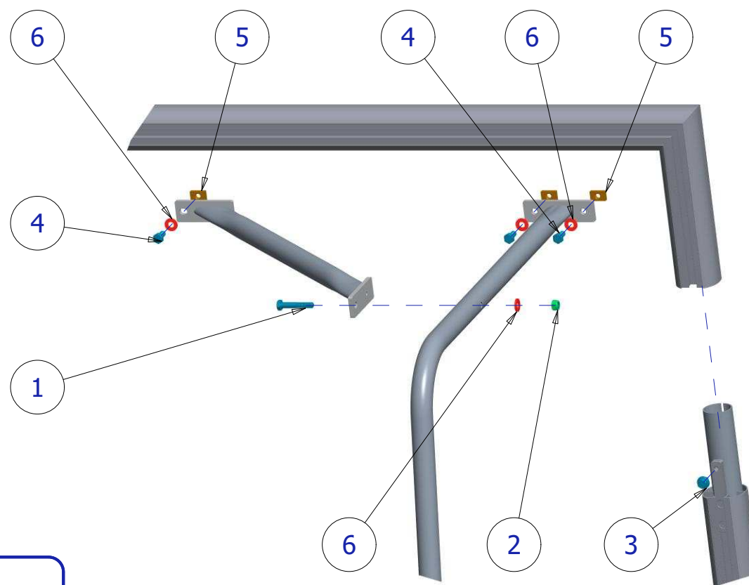
DETAIL C
