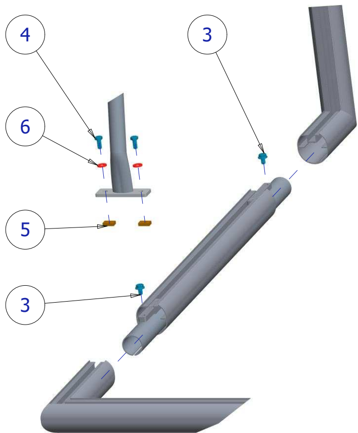
DETAIL B
