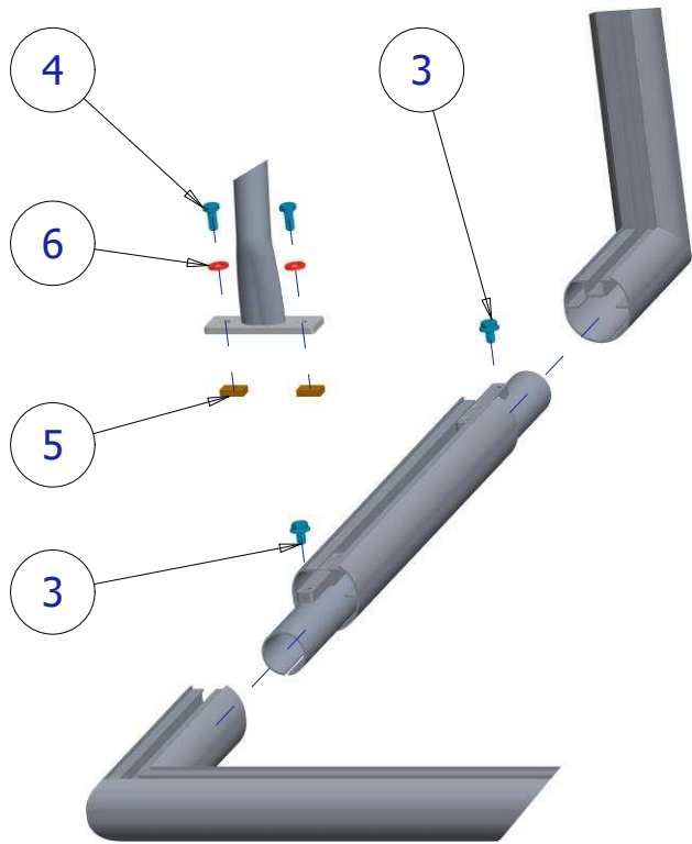
DETAIL B
