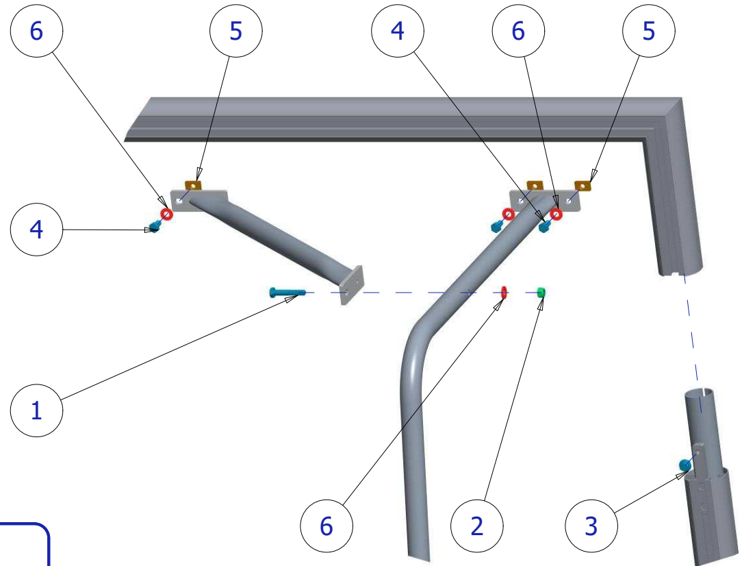
DETAIL C
