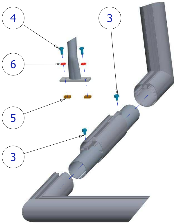
DETAIL B
