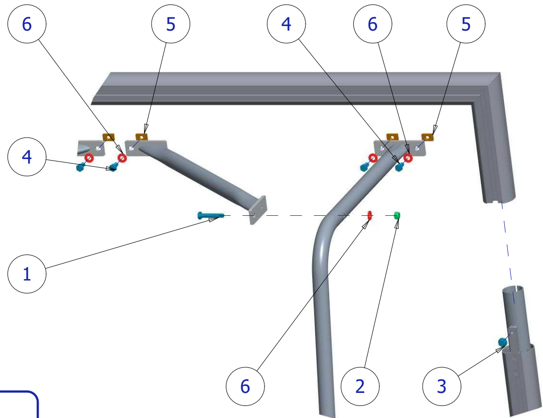
DETAIL C
