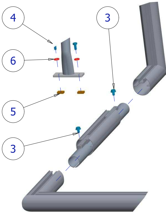
DETAIL B
