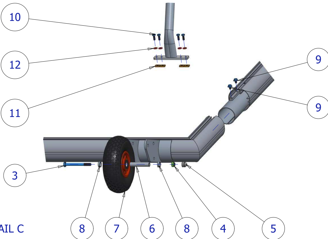
DETAIL B
