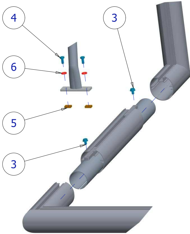
DETAIL B
